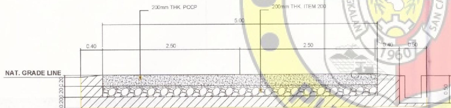
TYPICAL ROAD SECTION SCALE 1 : 50
