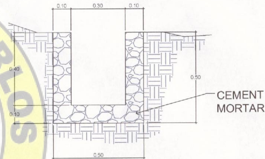
SECTION DETAILS SCALE 1 : 25
